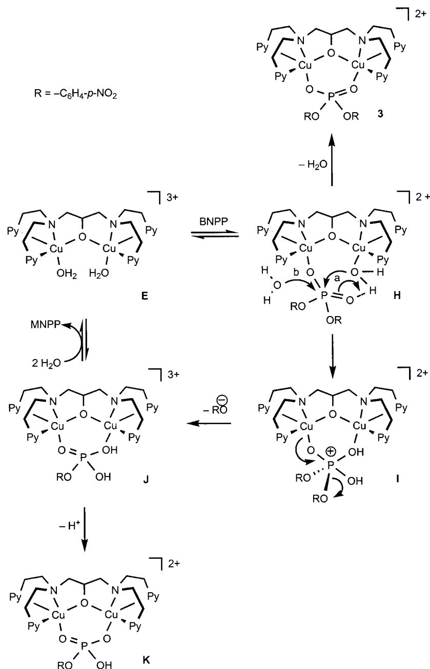
Scheme 4. Proposed mechanism for BNPP hydrolysis promoted by the copper complex 2 .
