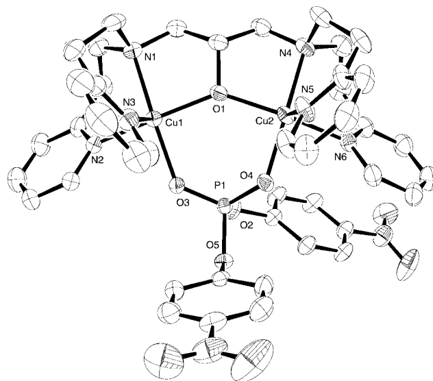
Figure 3. ORTEP perspective view of the copper(II) complex [\text{Cu}_2(\text{L}^2\text{O})(\text{BNPP})](\text{CF}_3\text{SO}_3)_2 ( 3 ). The H atoms and 2 \text{CF}_3\text{SO}_3^- counterion are omitted for clarity. Bond lengths are in Å: Cu1–O1 1.9823(3), Cu1–O3 1.9854(3), Cu1–N1 2.0628(4), Cu1–N2 2.0116(4), Cu1–N3 2.2432(4), Cu2–O1 1.9874(3), Cu2–O4 1.9733(3), Cu2–N4 2.0595(4), Cu2–N5 2.1864(4), Cu2–N6 2.0230(4). Bond angles are in °: O1–Cu1–O3 92.409(13), O1–Cu1–N1 86.28(2), O1–Cu1–N2 161.41(2), O1–Cu1–N3 102.662(14), O3–Cu1–N1 169.72(2), O3–Cu1–N2 86.358(15), O3–Cu1–N3 94.77(2), N1–Cu1–N2 91.63(2), N1–Cu1–N3 95.47(2), N2–Cu1–N3 95.92(2), O1–Cu2–O4 92.451(12), O1–Cu2–N4 86.62(2), O1–Cu2–N5 106.976(14), O1–Cu2–N6 157.079(15), O4–Cu2–N4 172.71(2), O4–Cu2–N5 91.56(2), O4–Cu2–N6 86.104(15), N4–Cu2–N5 95.63(2), N4–Cu2–N6 91.93(2), N5–Cu2–N6 95.93(2). Numbers in parentheses are the estimated standard deviation in the least significant digits.
