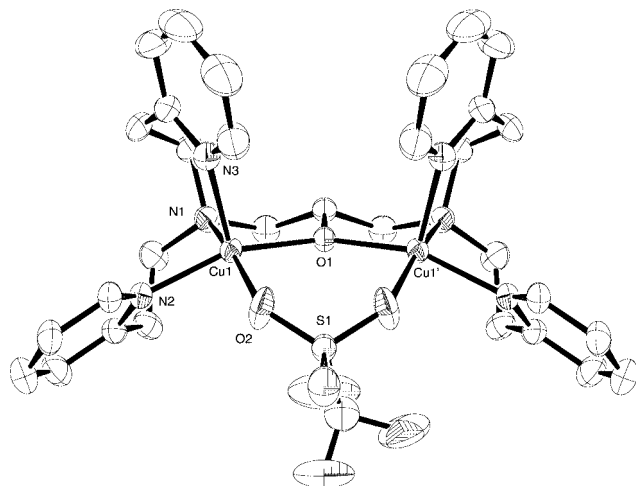
Figure 2. ORTEP perspective view of the copper(II) complex [\text{Cu}(\text{L}^2\text{OH})](\text{CF}_3\text{SO}_3)_2 ( 2 ). The H atoms and 2 \text{CF}_3\text{SO}_3^- counterion are omitted for clarity. Bond lengths are in Å: Cu1–O1 1.9695(12), Cu1–N2 2.009(3), Cu1–N1 2.032(3), Cu1–O2 2.047(3), Cu1–N3 2.179(4). Bond angles are in °: O1–Cu1–N2 159.45(14), O1–Cu1–N1 87.04(12), N2–Cu1–N1 94.17(12), O1–Cu1–O2 90.54(12), N2–Cu1–O2 83.10(13), N1–Cu1–O2 165.31(15), O1–Cu1–N3 104.69(11), N2–Cu1–N3 95.40(10), N1–Cu1–N3 98.93(14), O2–Cu1–N3 95.71(16). Numbers in parentheses are the estimated standard deviation in the least significant digits.
