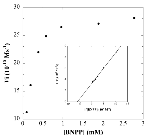
Figure 10. Saturation kinetics of copper complex 2 by BNPP. Each reaction mixture contained 50 mM MES/0.1 M KCl, pH 6 at 40 °C and 0.5 mM 2 . Inset: Lineweaver–Burk plot, the plotted line is the computer-generated best fit ( R = 0.9978 ) according to 1/V_i = K_M/(V_{max}[\text{BNPP}]) + 1/V_{max} , where K_M = 0.17 mM, V_{max} = 3.07 \cdot 10^{-9} \text{ M s}^{-1} and k_{cat} = 11.2 \cdot 10^{-6} \text{ s}^{-1} , \{[\text{L}^2\text{O}]\text{Cu}_2(\text{H}_2\text{O})_2\}^{3+} = 0.55[2] .
