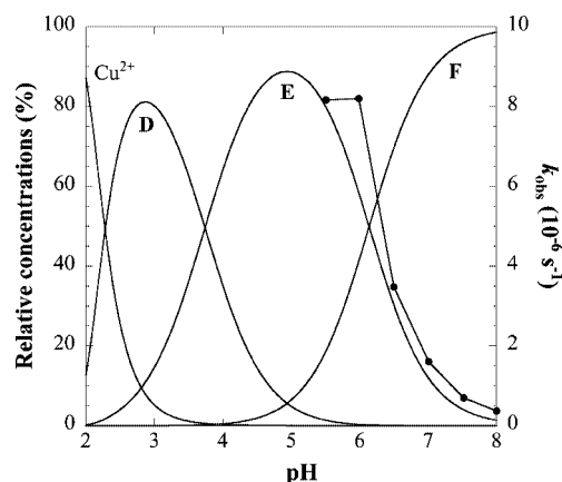
Figure 6. Species distribution of the complexes of L^2OH (5 mM) with 2 equiv. Cu^{2+} in 0.2 M KCl at 40 °C and pH/rate profile for BNPP hydrolysis promoted by 2 ; [2] = 0.488 mM, [BNPP] = 0.192 mM at 40 °C.
