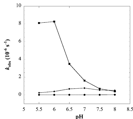
Figure 8. pH dependence on k_{\text{obs}} for BNPP hydrolysis promoted by copper complexes 1 (filled diamond) and 2 (filled square) and un-promoted (filled circle).
