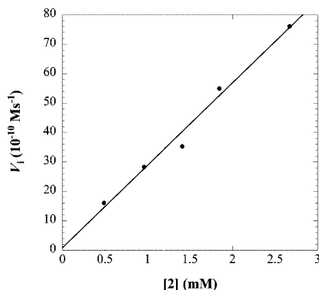
Figure 9. V_i vs. [2] of hydrolysis of BNPP. Each reaction mixture contained 50 mM MES/0.1 M KCl, pH 6 at 40 °C and 0.192 mM BNPP. The plotted lines are the computer-generated best fit with R = 0.9920 .
